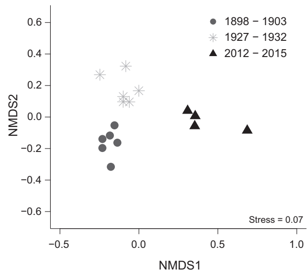
Figure 2: Ordination of the Lincoln Park (Chicago, IL) bird community across all survey years, showing the solution of nonmetric multidimensional scaling (NMDS). Distances among the bird communities each year were measured with the Bray-Curtis index.
